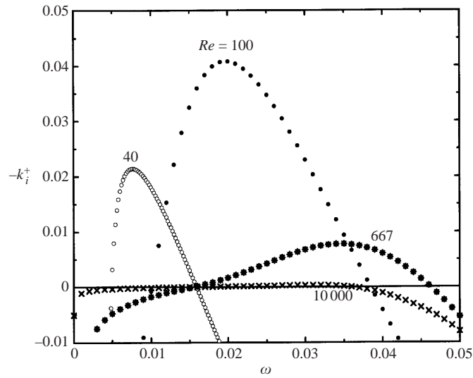
FIGURE 7. Spatial growth rate -k_i^+ of viscous bending mode m = +1 versus real frequency \omega for different Reynolds numbers Re at a = 0 , q = 0.4 . \circ , Re = 40 ; \bullet , Re = 100 ; * , Re = 667 ; \times , Re = 10000 .
